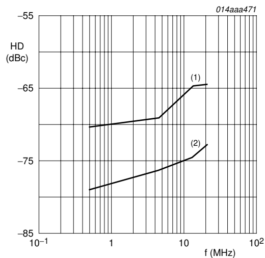
Fig 6. Harmonic Distortion (HD) as a function of frequency for minimum gain
