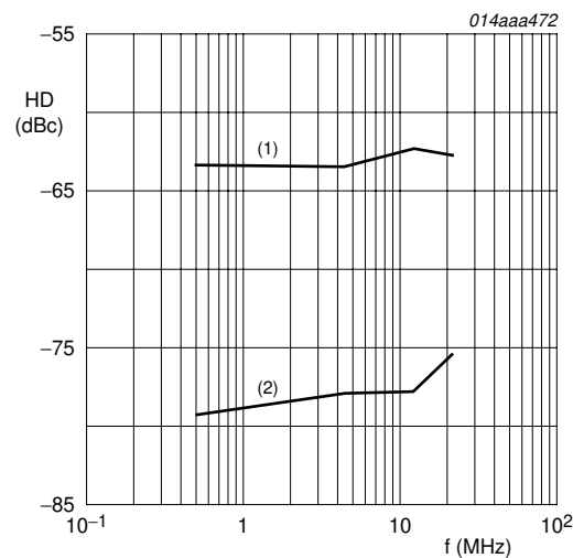
Fig 7. Harmonic Distortion (HD) as a function of frequency for minimum gain plus 6 dB
