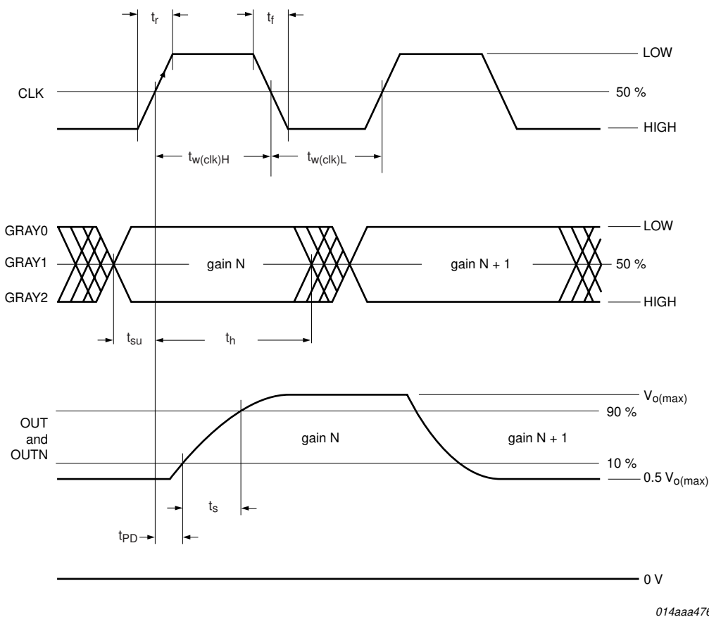
Fig 3. Latched mode timing diagram
